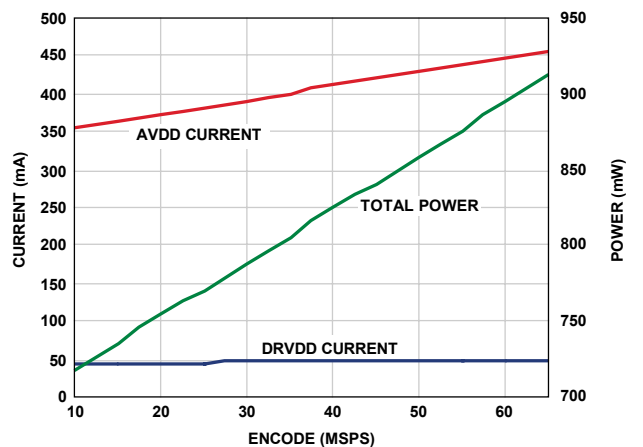
Figure 70. Supply Current vs. f_{SAMPLE} for f_{IN} = 10.3 MHz, AD9222- 65
