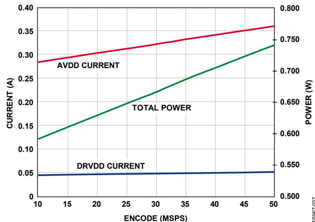
Figure 69. Supply Current vs. f_{SAMPLE} for f_{IN} = 10.3 MHz, AD9222- 50
